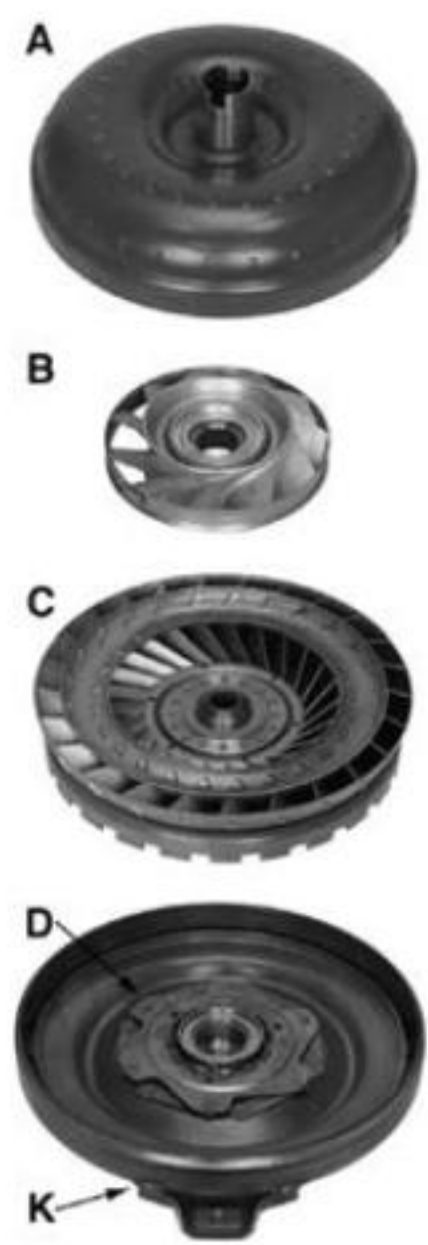
Lock Up Captive Clutch
