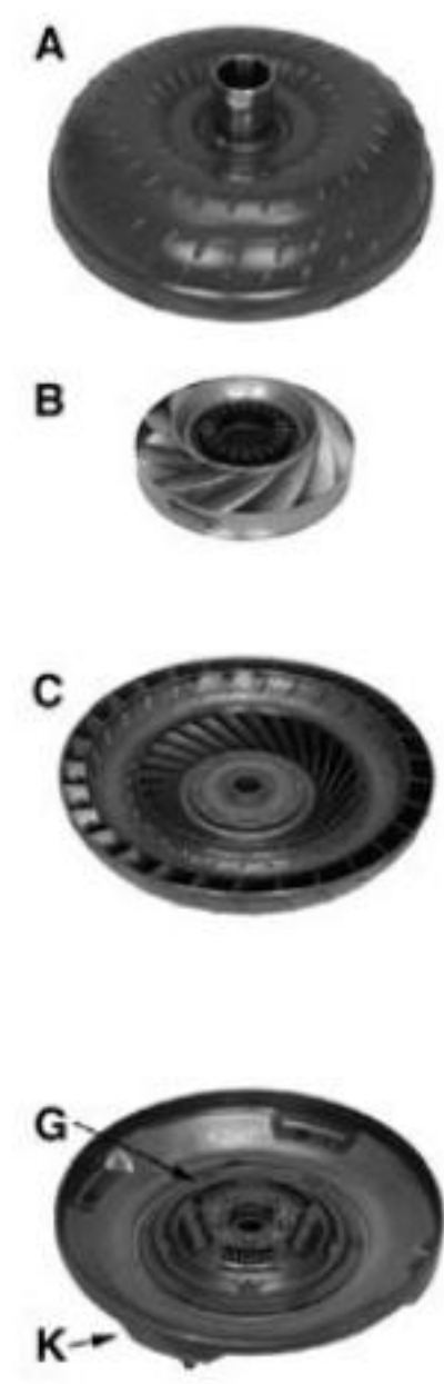
Lock Up Damper Drive
