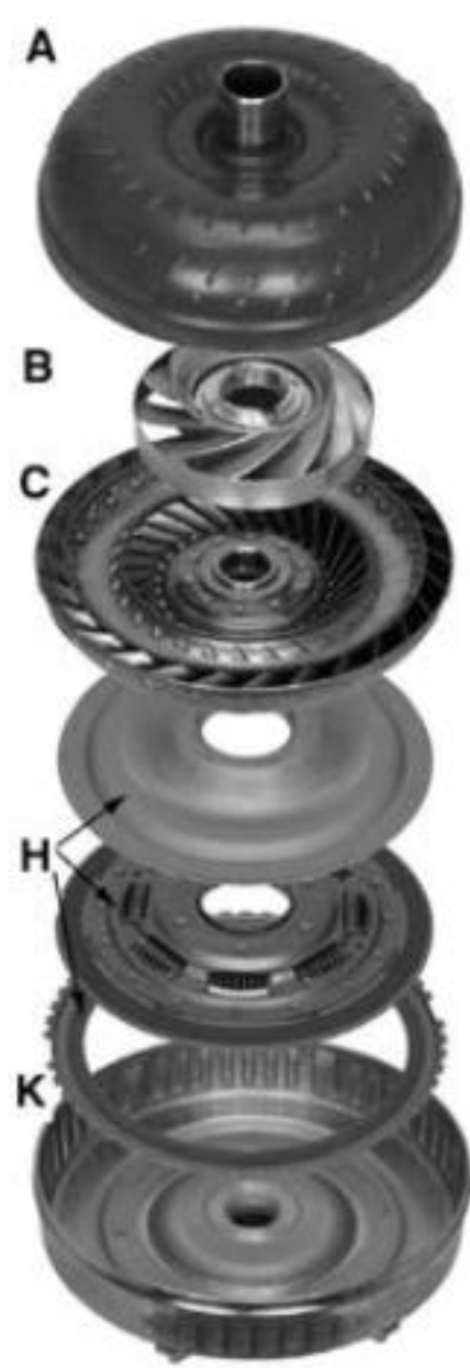
Lock Up Multi Friction Clutch
