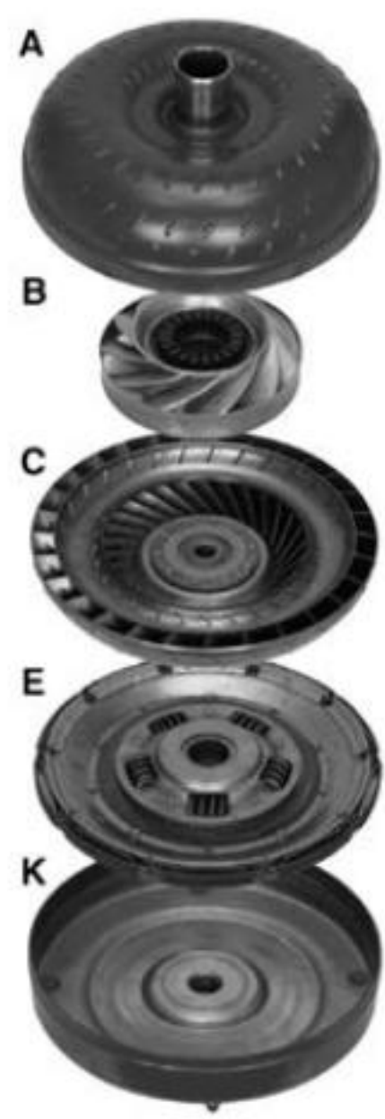
Lock Up Centrifugal Clutch
