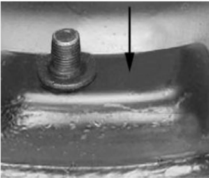
Boss
