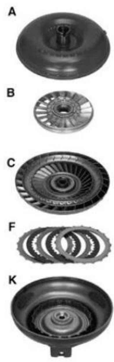
Lock Up Clutch Pack
