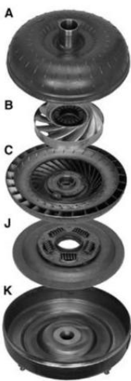
Lock Up Piston (Single Friction Clutch)
