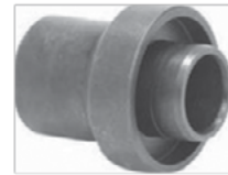
T-1208 Axle Shaft Seal Use with Driver Handle T-1093 Fits Nissan JF403E & GM-Geo
