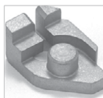
T-2901 Adapter Use with Transmission Holding Fixture T-0156-B
