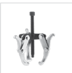
T3907 5 Ton Capacity 2 or 3 Jaw Gear Puller Maximum Reach 3.325" Maximum Spread 4.75" Reversible Jaws
